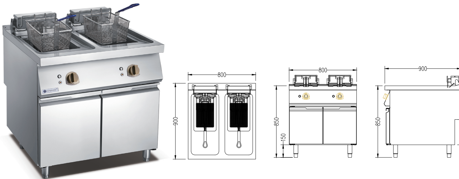
电力炸炉下连掩门柜 Electric Fryer With Cabinet
